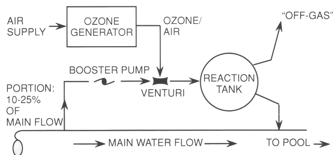
FIGURE 1—Slipstream ozonation
