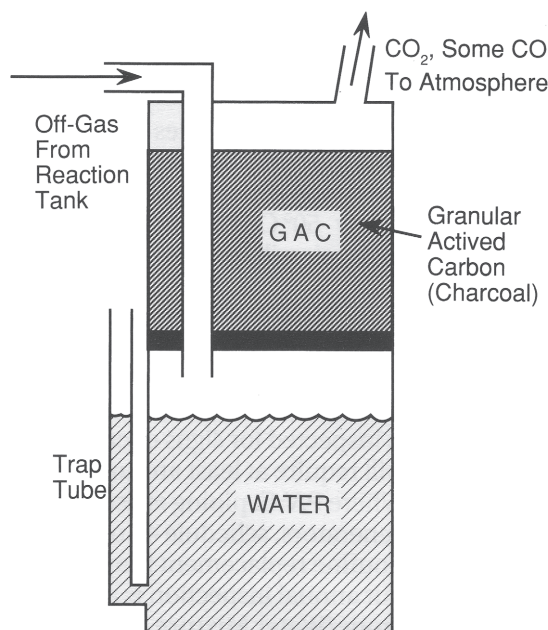
FIGURE 3—Ozone destructor
